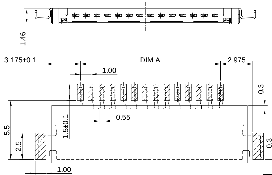
PCB LAYOUT
