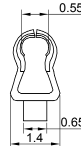
SEC:C-C
