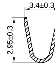
SEC B-B
