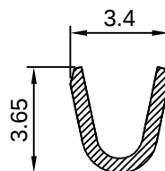
SEC B-B
